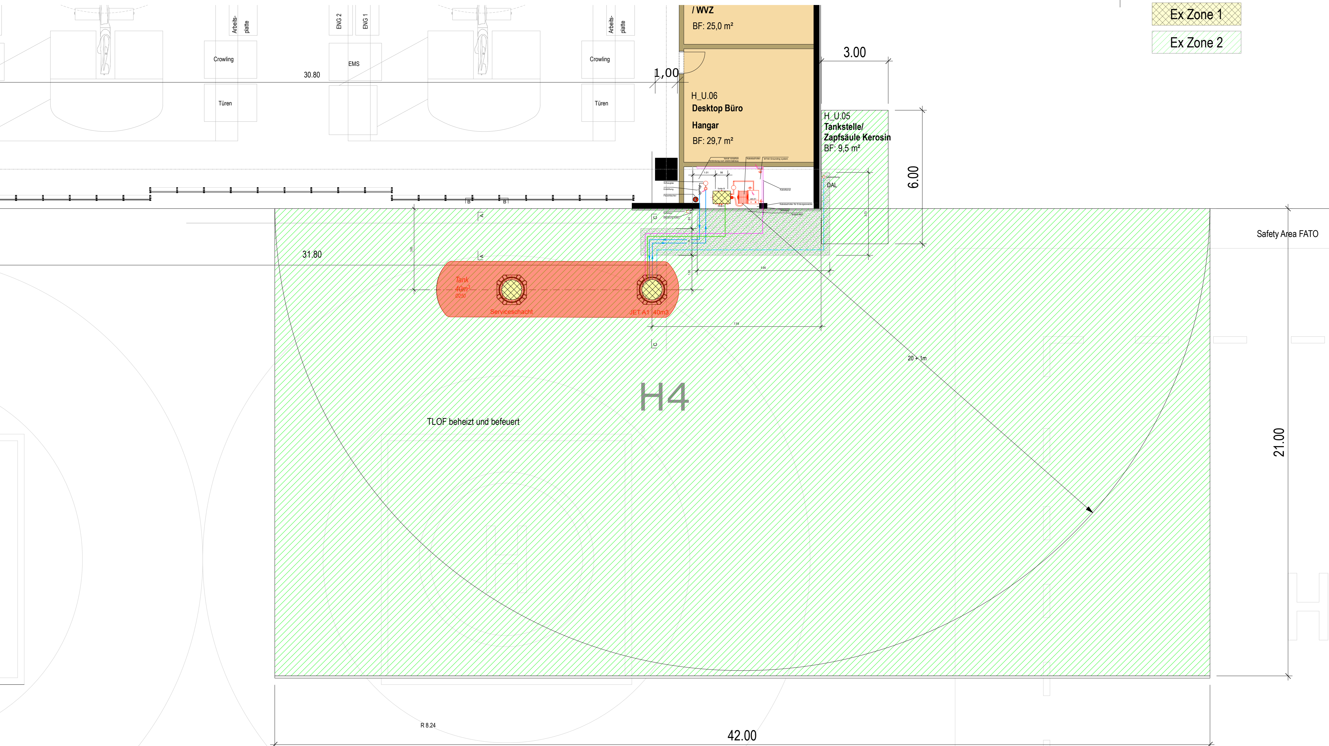
Situation Ech. 1/100
